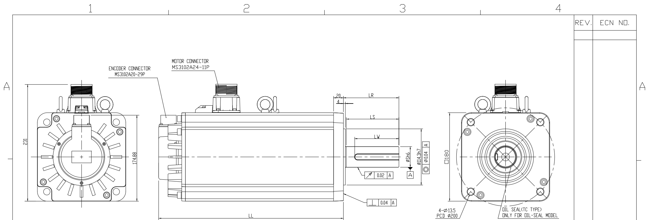
DIMENSION TABLE (MODEL WITH BRAKE)
