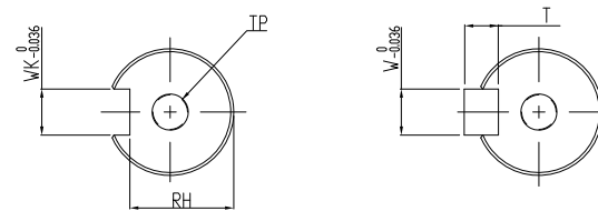
SHAFT END DETAILS
