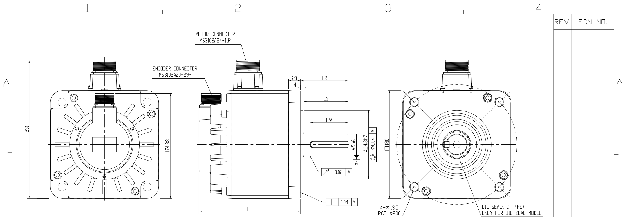
DIMENSION TABLE (MODEL WITHOUT BRAKE)
