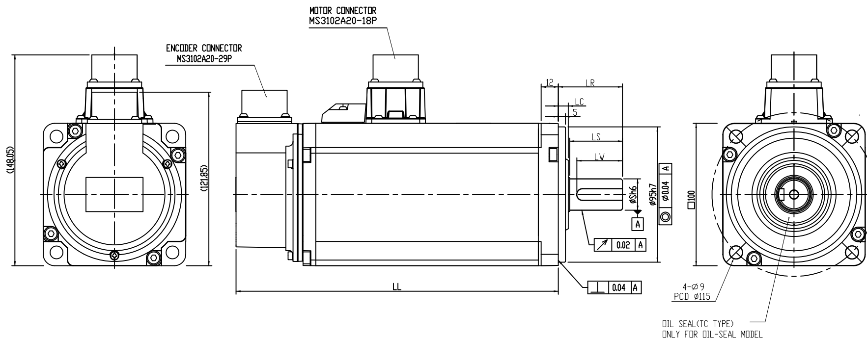
DIMENSION TABLE (MODEL WITH BRAKE)
