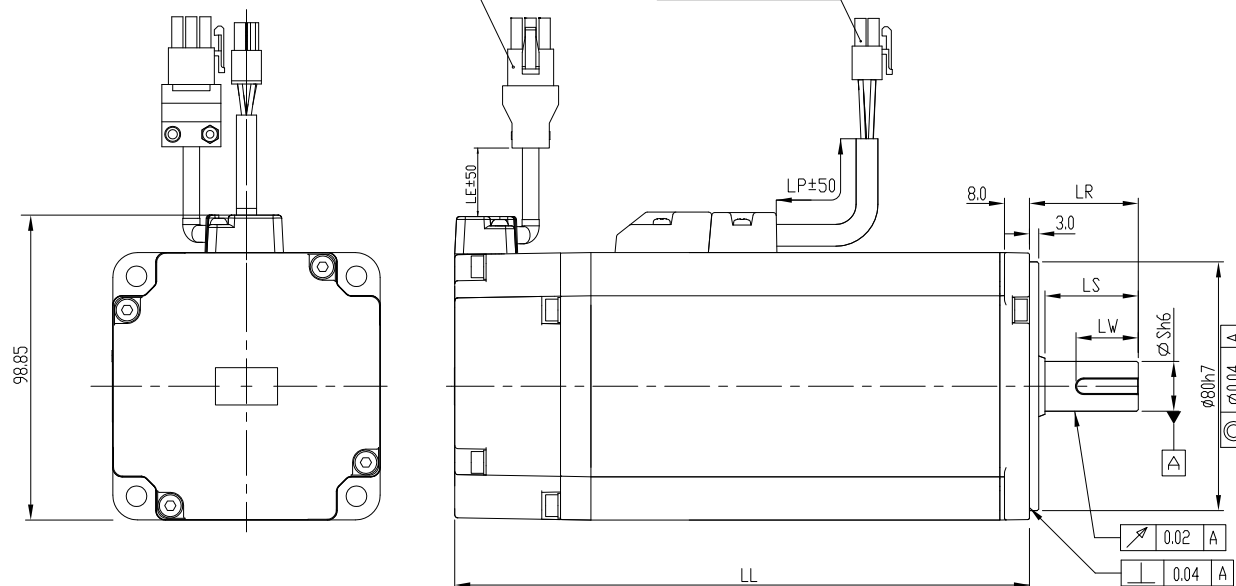
DIMENSION TABLE (MODEL WITH BRAKE)
