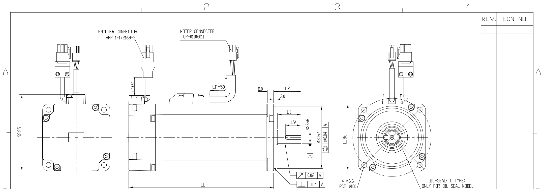
DIMENSION TABLE (MODEL WITH BRAKE)
