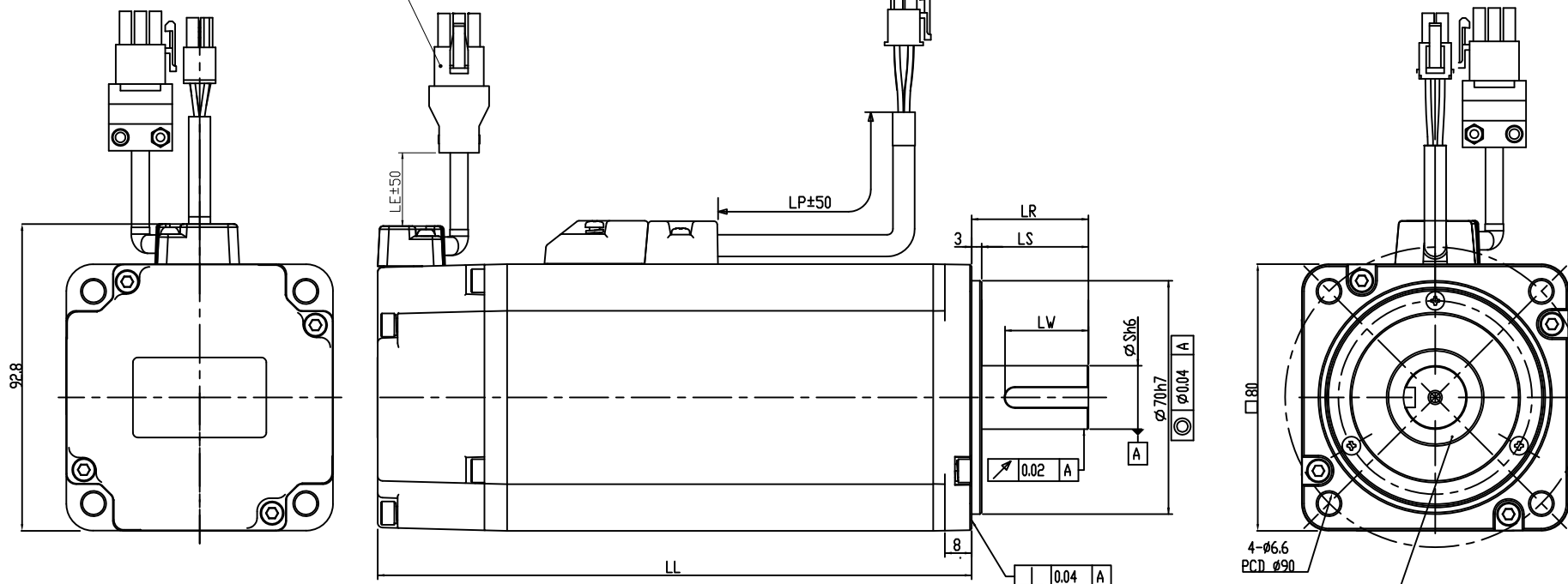
DIMENSION TABLE (MODEL WITH BRAKE)
