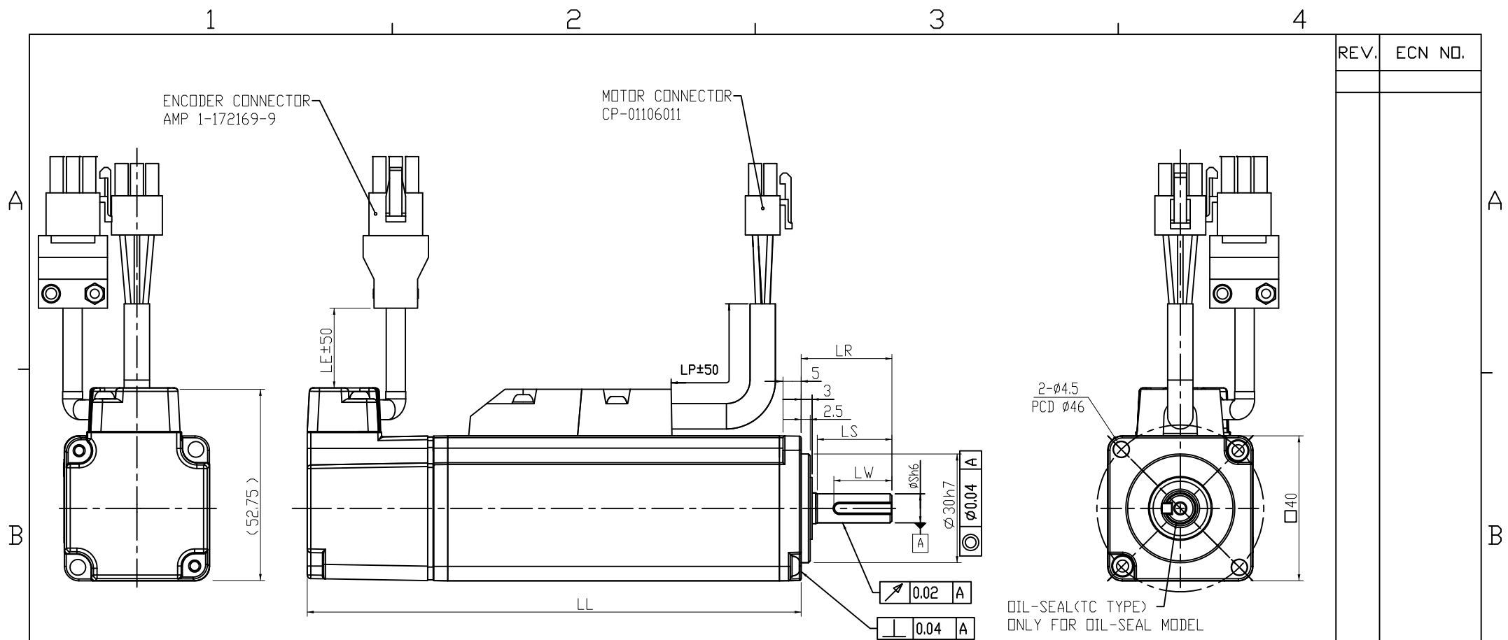
DIMENSION TABLE (MODEL WITH BRAKE)
