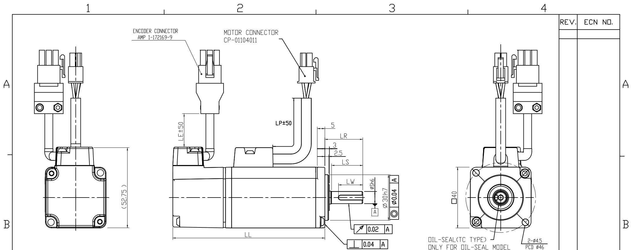
DIMENSION TABLE (MODEL WITHOUT BRAKE)
