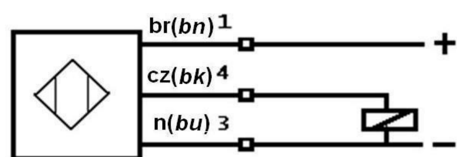
PNP
